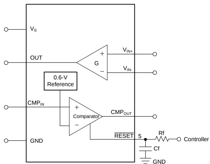
Figure 31. Filter on RESET Pin
