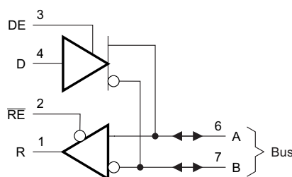
Figure 13. Half-Duplex Transceiver
