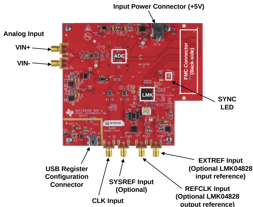
Figure 1. EVM Feature Locations
