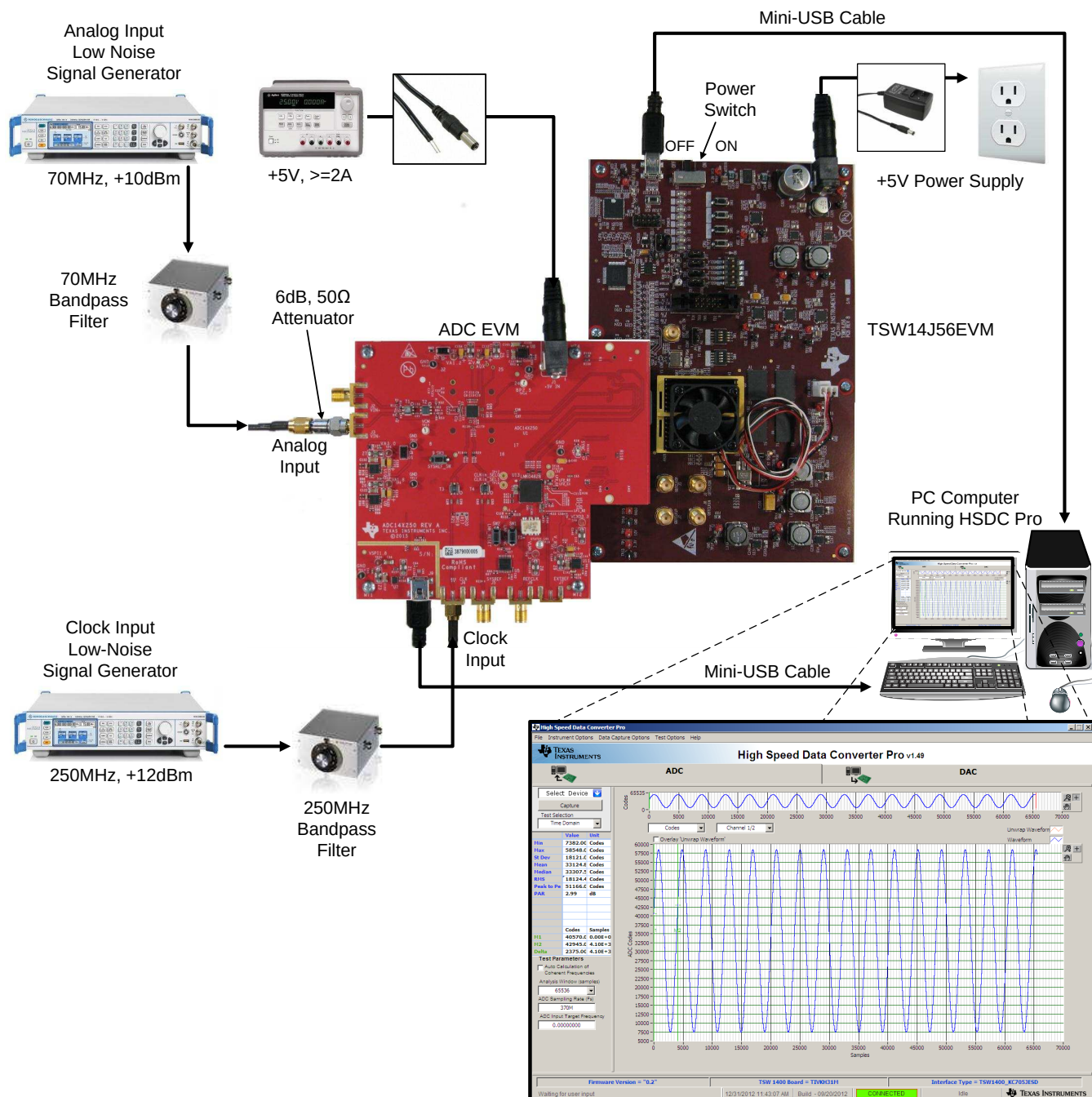
Figure 2. Quick Start Test Setup
