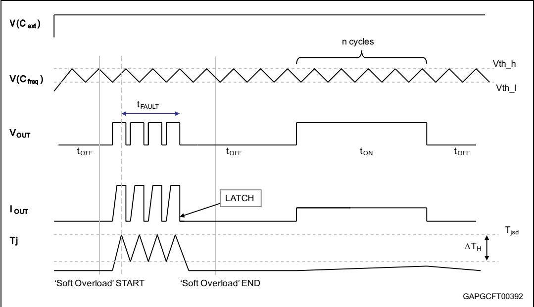
Figure 8. Thermal limitation event duration > t_{FAULT}
