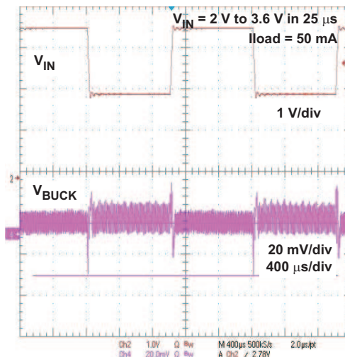
Figure 13. Buck Output Line Transient Response
