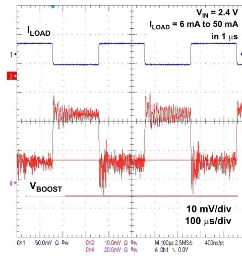
Figure 15. Boost Load Transient Response
