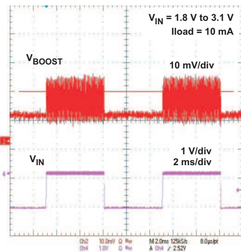
Figure 14. Boost Line Transient Response
