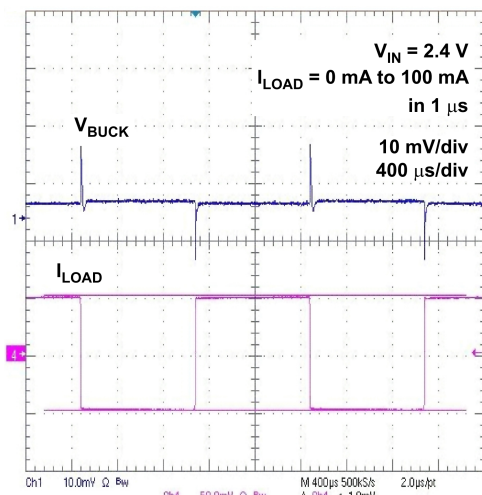
Figure 12. Buck Output Load Transient Response
