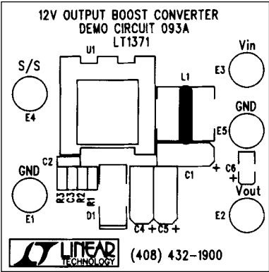
Silkscreen Top
