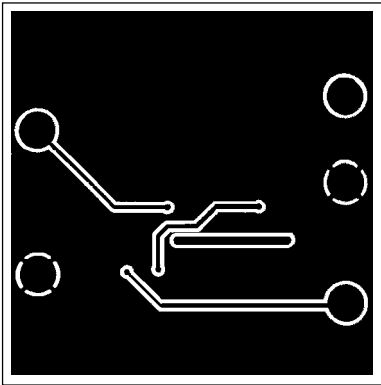
Solder Side
