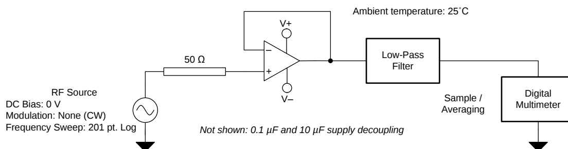
Figure 43. EMIRR +IN Test Configuration
