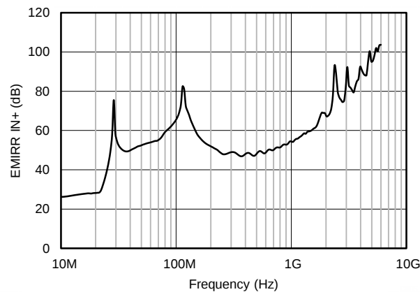
Figure 42. EMIRR Testing
