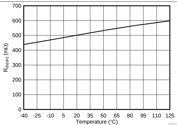
Figure 5. Rectifier On Resistance vs Temperature
