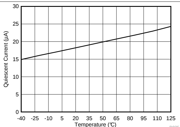
Figure 3. I_Q into VMAIN Pin at Active Mode vs Temperature
