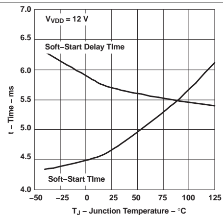
Figure 11. Soft Start Timing vs Temperature
