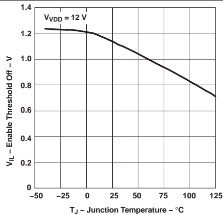
Figure 9. Enable Threshold Off vs Temperature
