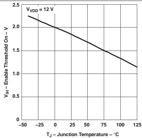
Figure 7. Enable Threshold On vs Temperature
