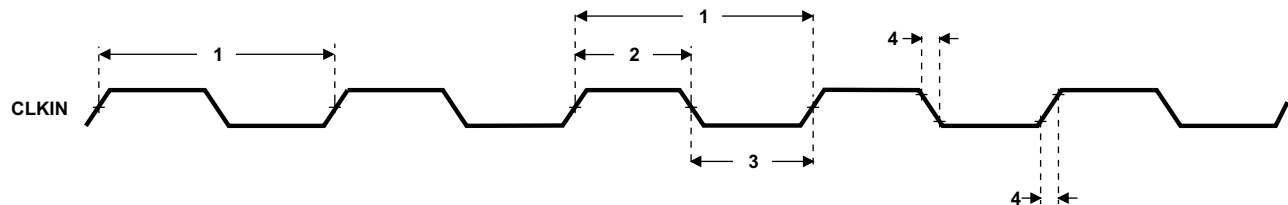
Figure 5-9. CLKIN Timing
