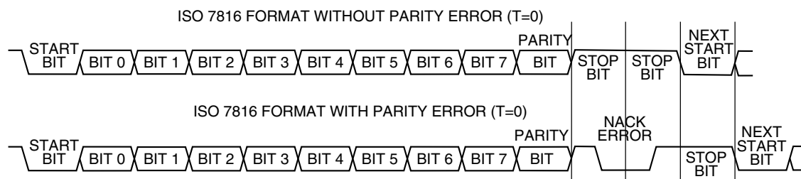
Figure 49-312. ISO-7816 T = 0 data format
