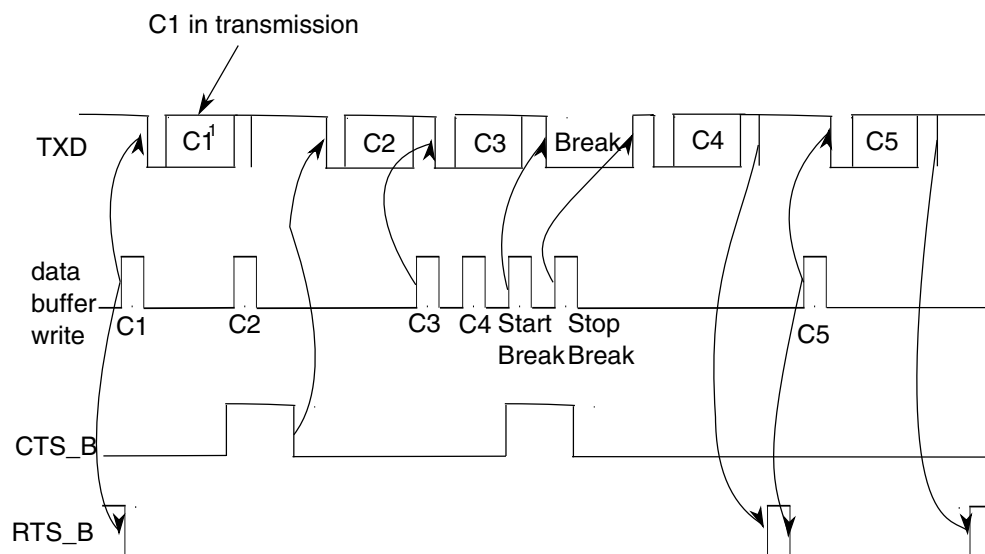
Figure 49-295. Transmitter RTS and CTS timing diagram
