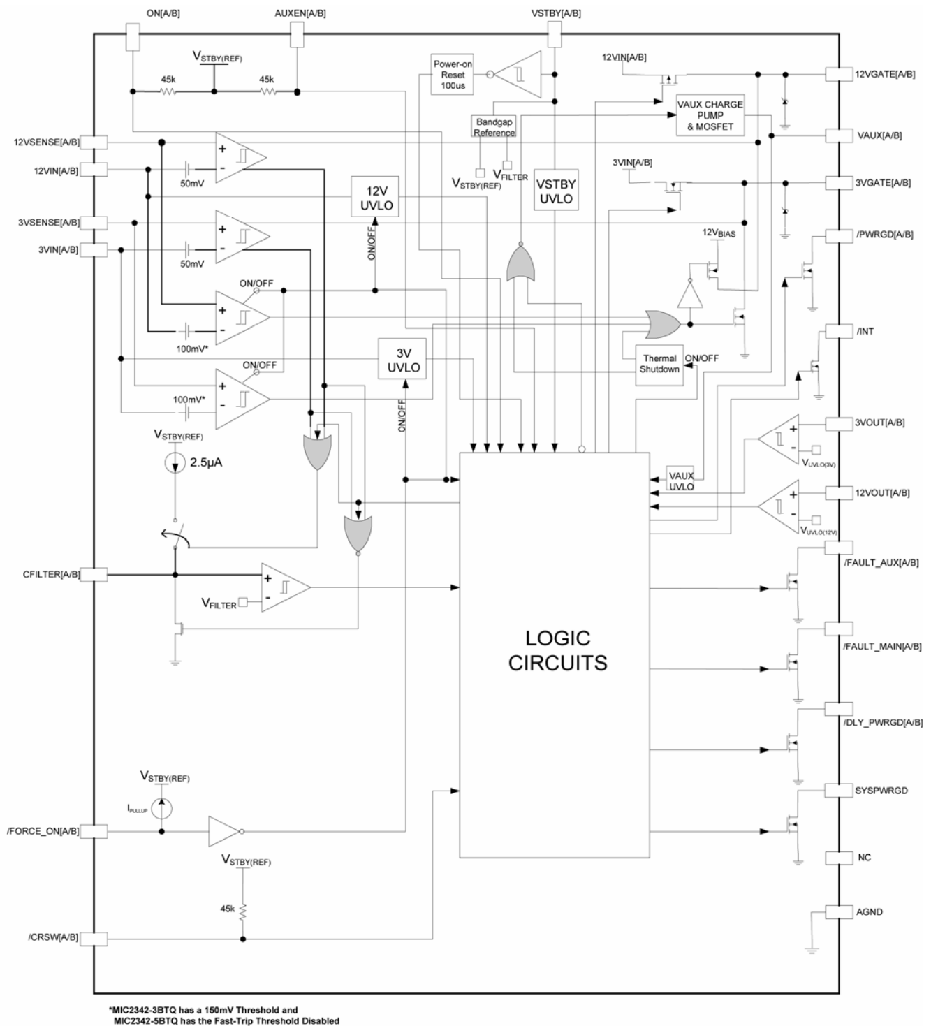
MIC2342/MIC2342R Block Diagram
