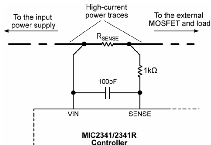
Figure 13. Current Limit Sense Filter for Noisy Systems
