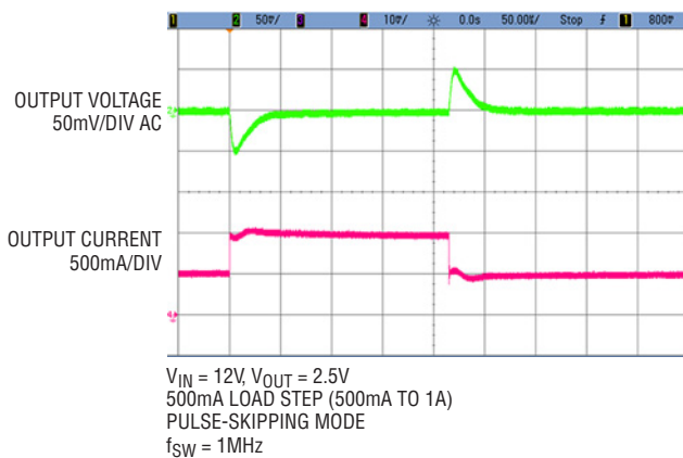
Figure 4. Load Step Response
