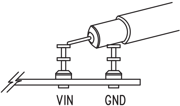
Figure 2. Measuring Input or Output Ripple
