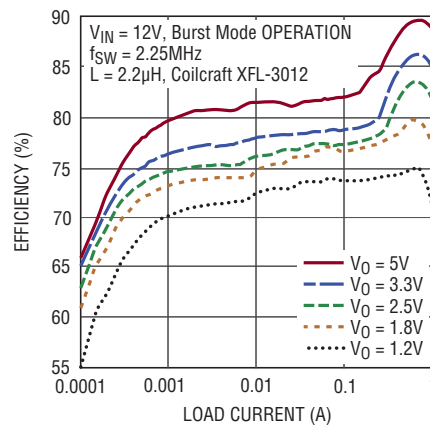
Figure 7. Circuit Efficiency
