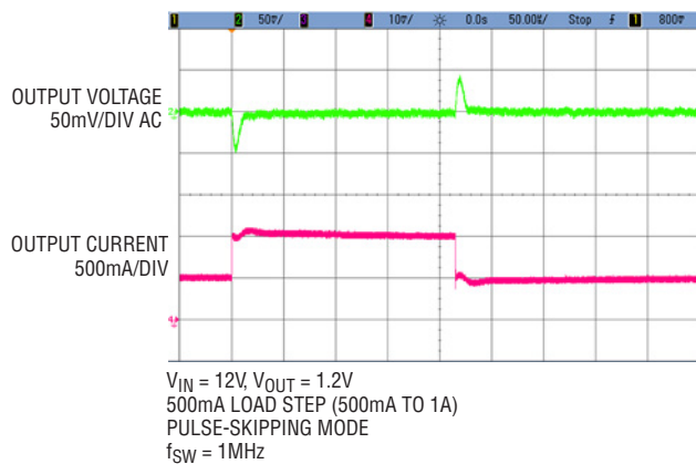
Figure 3. Load Step Response
