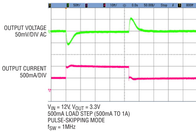
Figure 5. Load Step Response
