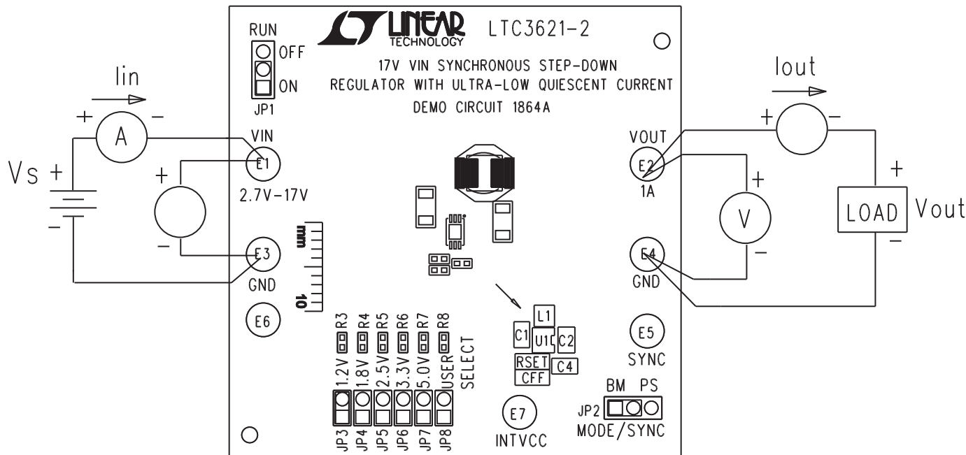
Figure 1. Proper Equipment Measurement Setup
