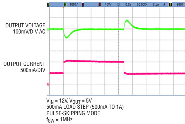
Figure 6. Load Step Response
