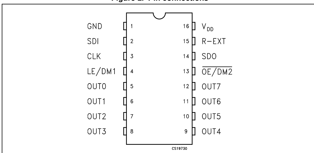
Figure 1. Pin connections
