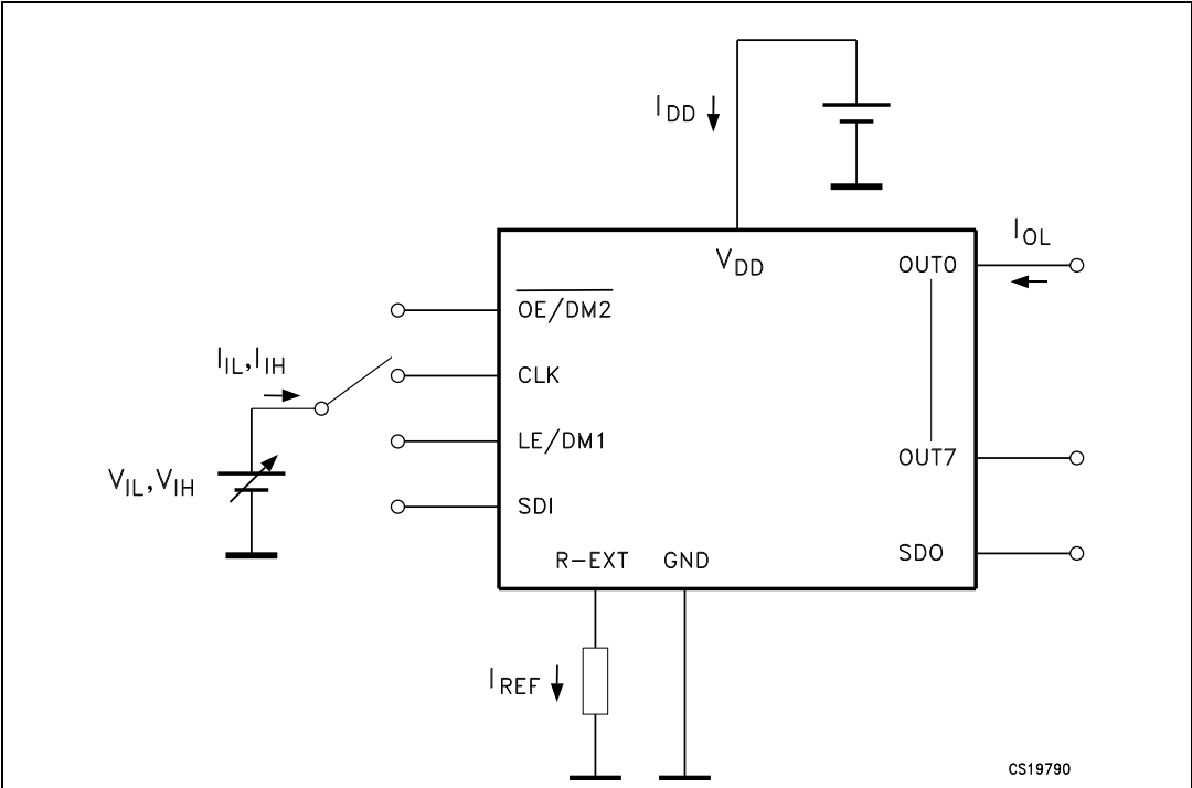
Figure 14. DC characteristics
