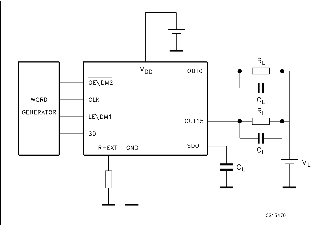
Figure 15. AC characteristics
