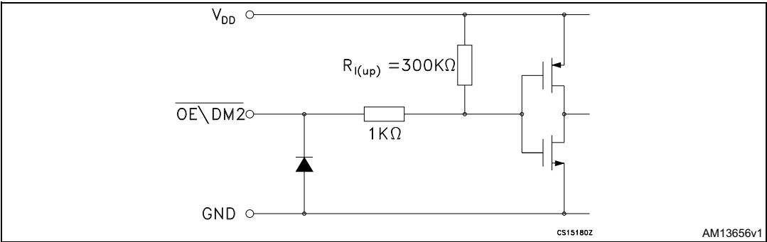
Figure 3. \overline{\text{OE}}/\text{DM2} terminal
