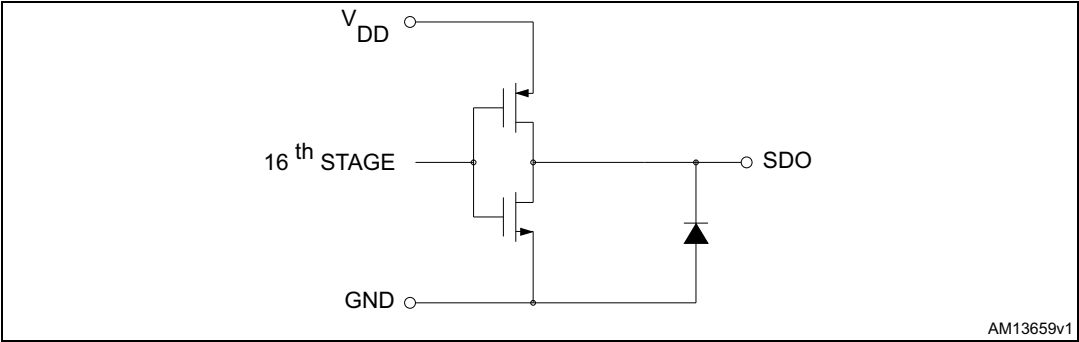
Figure 6. SDO terminal
