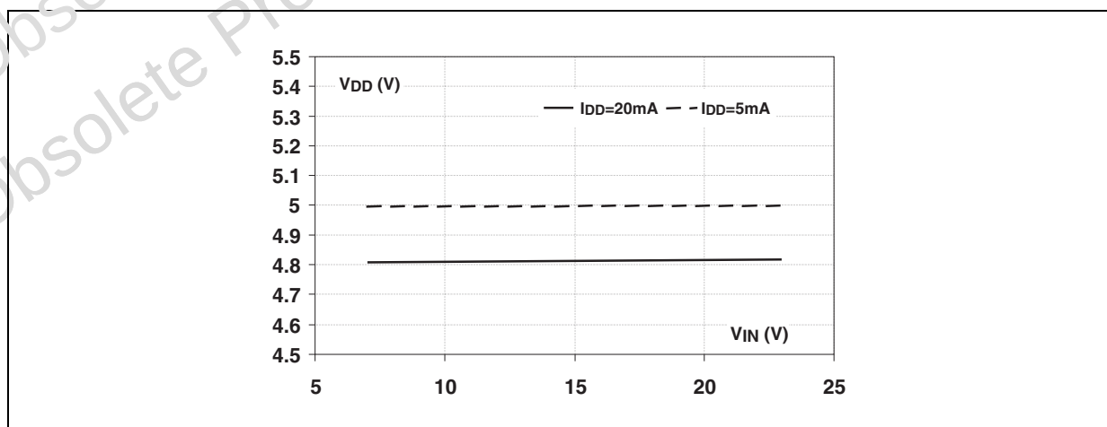
Figure 6: Regulator output voltage versus its input voltage with I_{DD} = 5 and 20 mA and T_J = 25^\circ\text{C}
