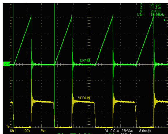
Figure 7. Drain current and voltage at max. load 90 V AC
