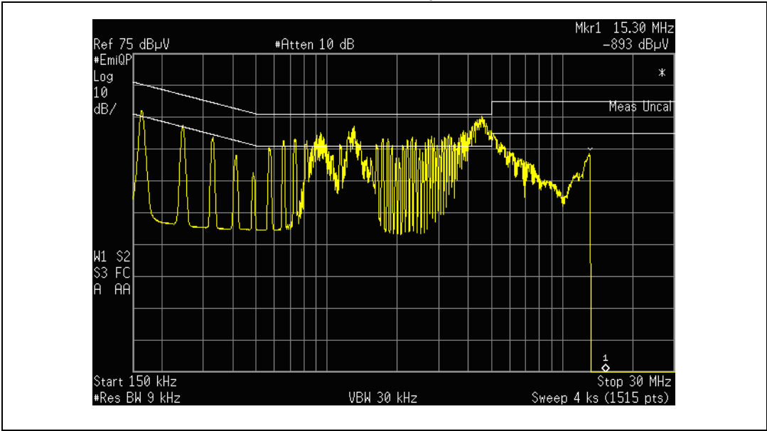
Figure 46. Quasi-peak measurement at 230 V AC - full load
