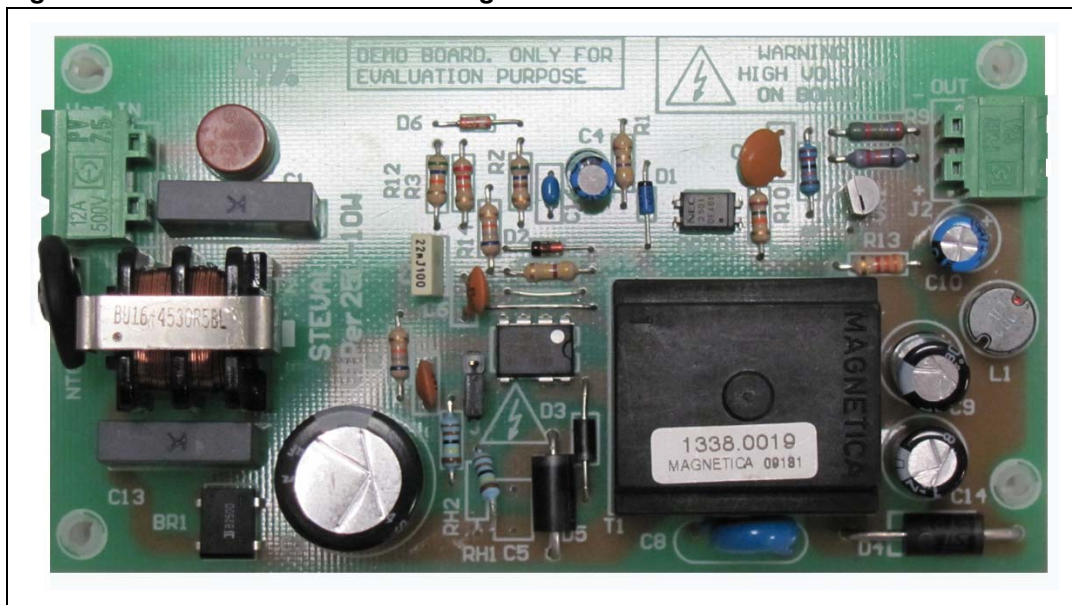
Figure 1. Demonstration board image
