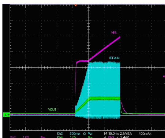
Figure 28. OLP: steady-state (auto-restart mode) - zoom
