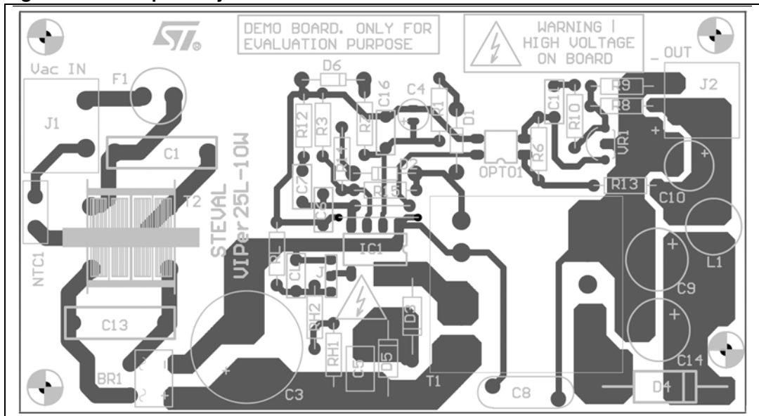
Figure 48. Complete layout
