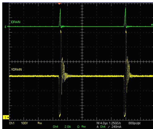
Figure 34. Operating with secondary winding shorted - restart mode – zoom2
