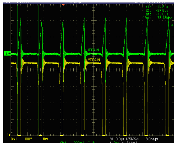
Figure 8. Drain current and voltage at max. load 265 V AC
