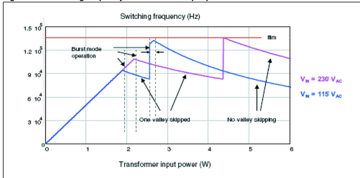
Figure 11. Switching frequency vs. transformer input power
