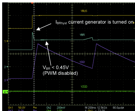
Figure 42. Input voltage steps from 60 V DC to 100 V DC - no turn-on
