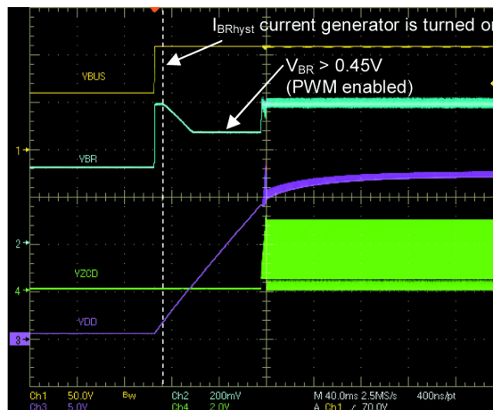
Figure 43. Input voltage steps from 60 V DC to 115 V DC - turn-on
