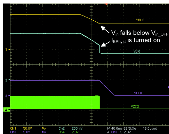
Figure 45. Input voltage steps from 115 V DC to 80 V DC - turn-off
