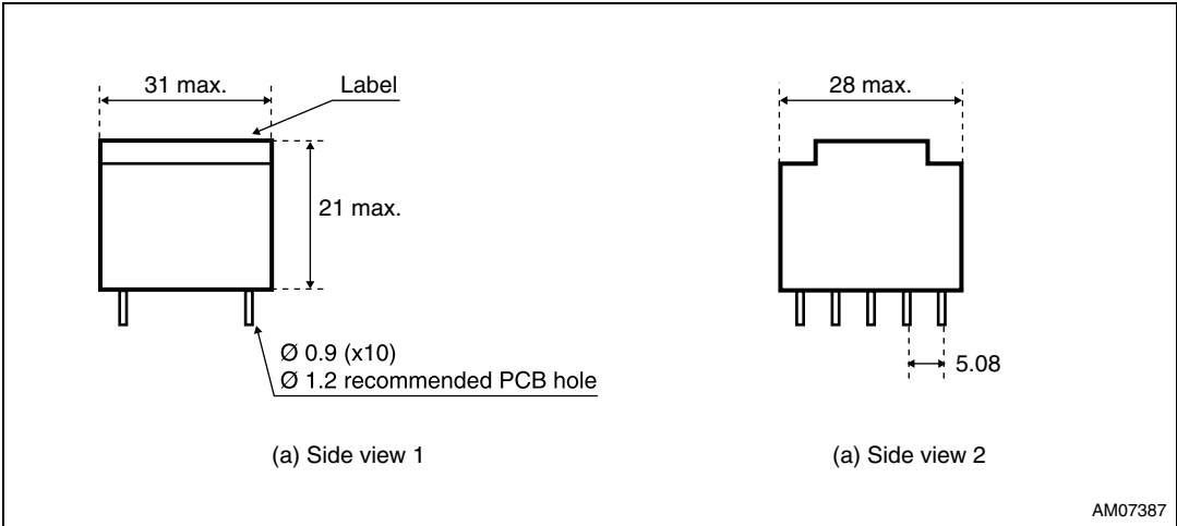
Figure 4. Transformer size
