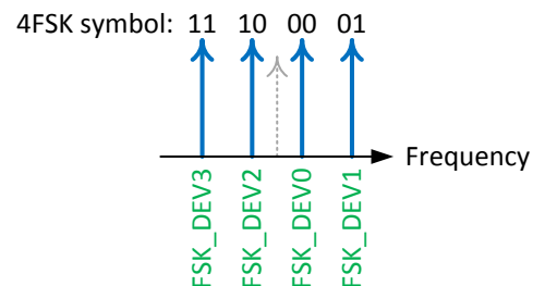
Figure 52. Typical 4FSK Definition
