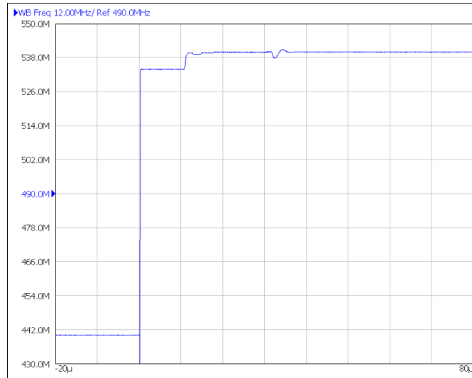
Figure 80. External VCO to Internal VCO Switching
