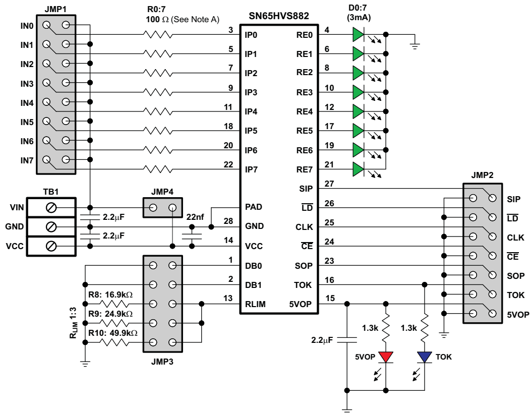
Figure 1. SN65HVS882EVM Schematic
