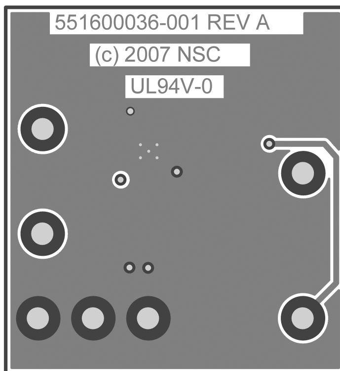
Figure 4. Bottom Layer
