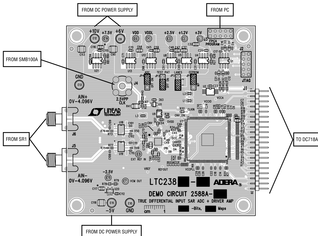
Figure 1. DC2588A Connection Diagram
