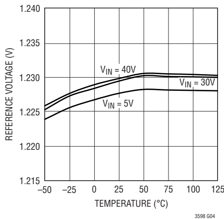
Reference Voltage
