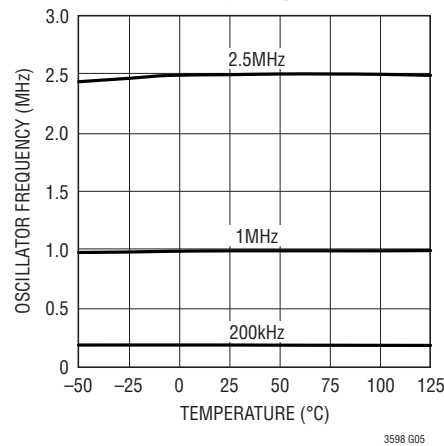
Oscillator Frequency
