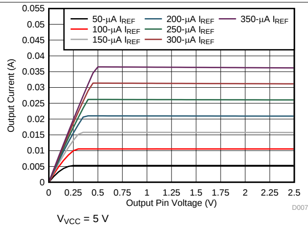
Figure 8. OUT Pin Voltage vs Current
