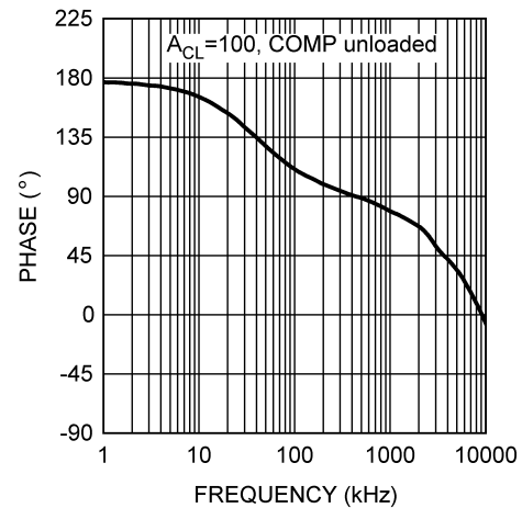
Figure 16. Error Amp Phase vs Frequency
