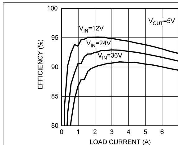
Figure 40. Efficiency With 6-μH Copper Inductor
