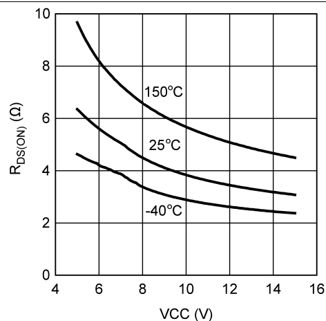
Figure 4. HO High R_{DS(ON)} vs VCC
