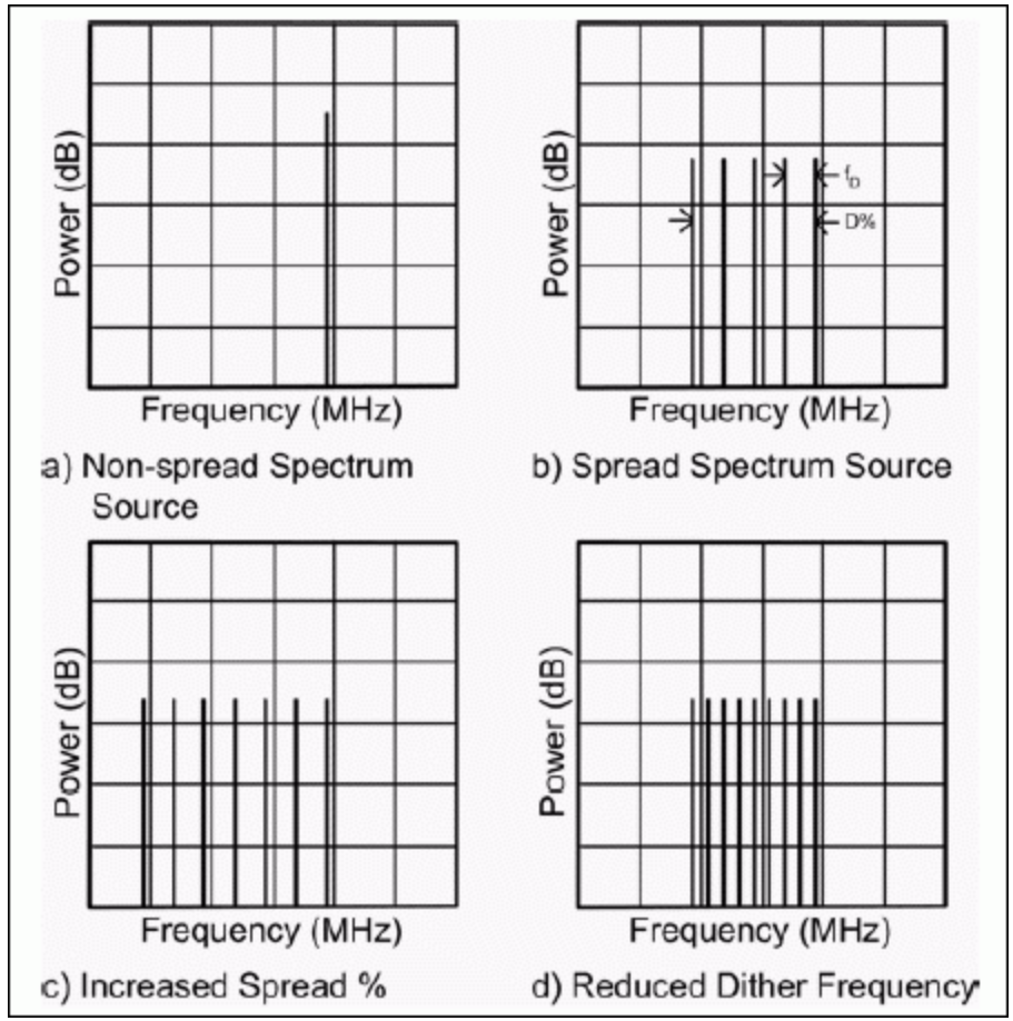
Figure 1. Spectral components of non-dithered and dithered oscillators.
