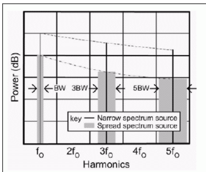
Figure 3. Spectral content for dithered oscillator harmonics.
