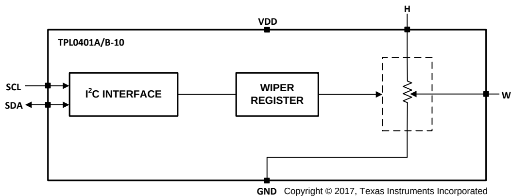
Simplified Schematic
