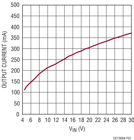
Figure 1. V_{OUT1} Typical Maximum Output Current vs V_{IN} When V_{OUT2} is not Loaded
