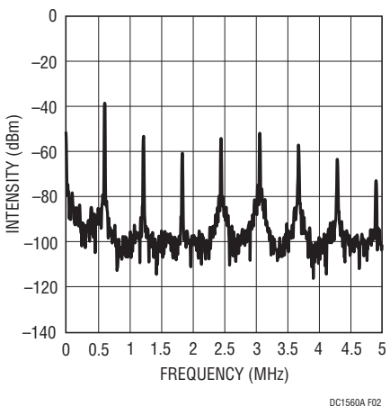
Figure 2. V_{OUT1} Output Noise Spectrum with I_{OUT2} at 100mA and V_{IN} at 12V ( V_{OUT1} Has no Extra Load)
