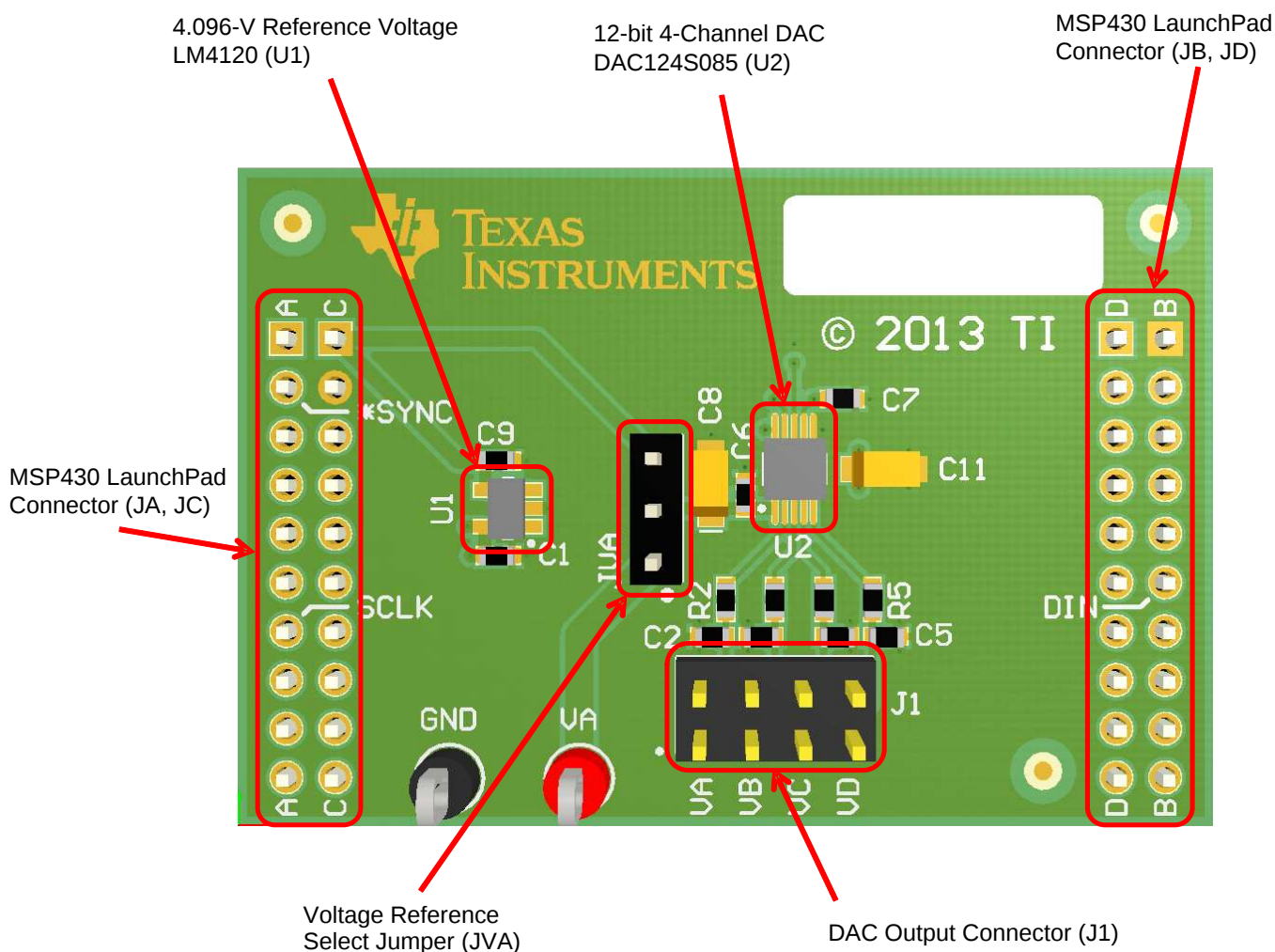
Figure 1. DAC124S085EVM Evaluation Board
