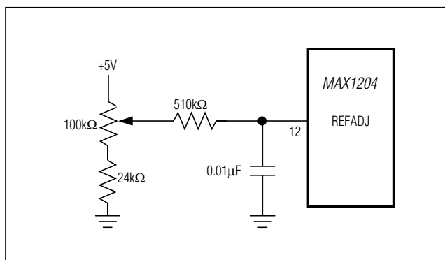
Figure 17. Reference-Adjust Circuit
