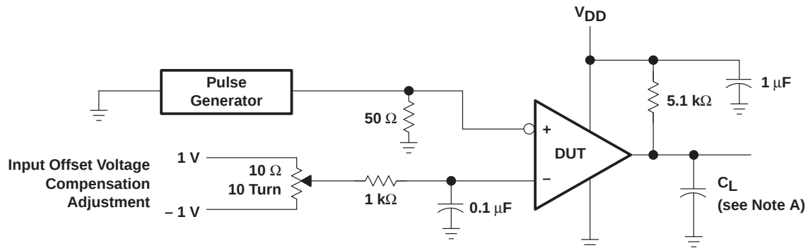
TEST CIRCUIT
