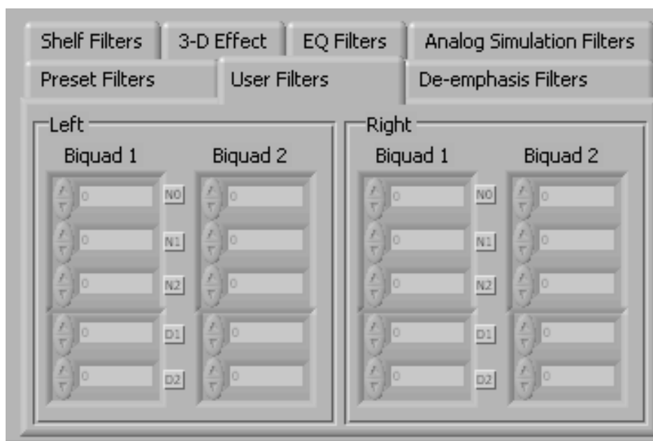
Figure 24. User Filters
