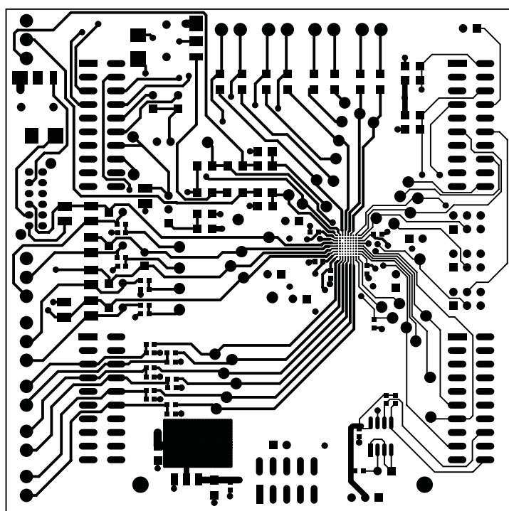
Figure 32. Top Layer
