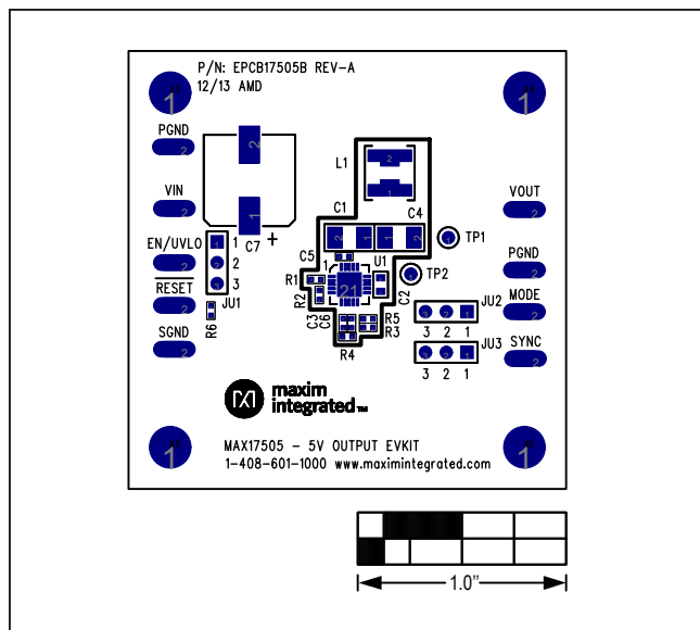
Figure 12. MAX17505 5V Output EV Kit Component Placement Guide—Component Side
