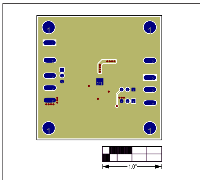
Figure 16. MAX17505 5V Output EV Kit PCB Layout—Solder Side
