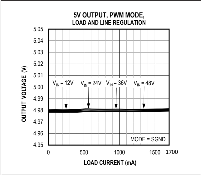
Figure 1. MAX17505 5V Output Load and Line Regulation (PWM Mode)
