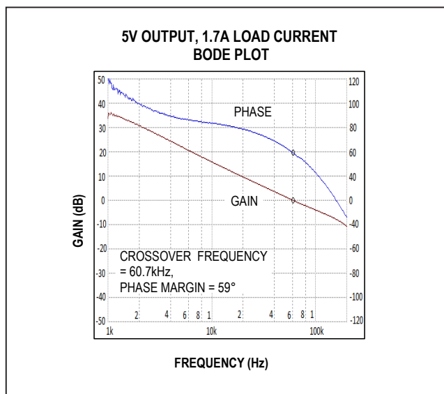
Figure 6. MAX17505 5V Output Full Load Bode Plot ( V_{IN} = 24V )
