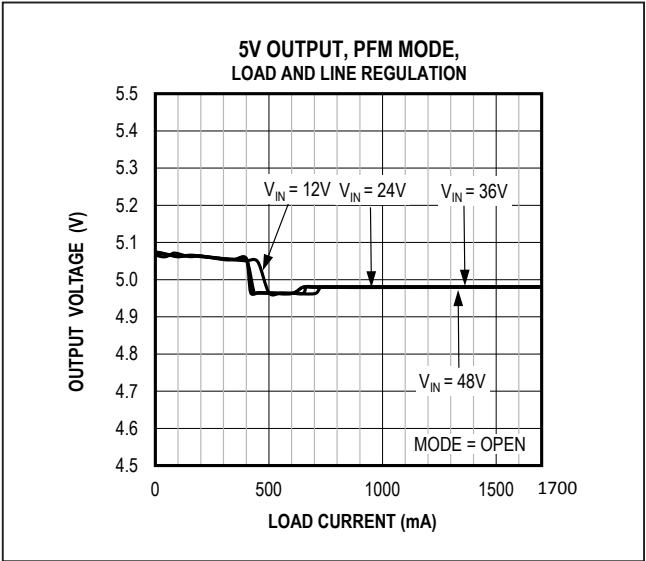
Figure 3. MAX17505 5V Output Load and Line Regulation (PFM Mode)
