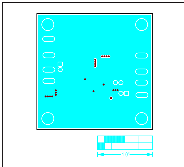
Figure 14. MAX17505 5V Output EV Kit PCB Layout—Inner Layer 1
