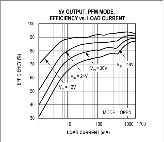
Figure 4. MAX17505 5V Output Efficiency (PFM Mode)
