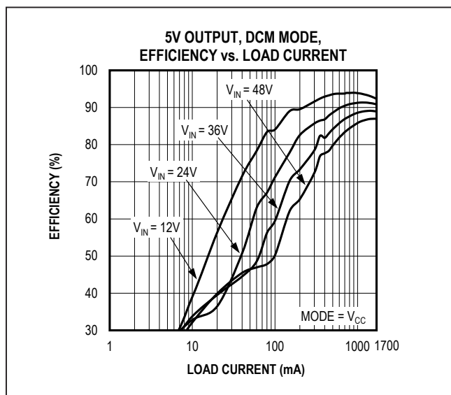
Figure 5. MAX17505 5V Output Efficiency (DCM Mode)
