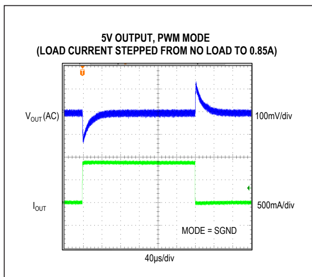
Figure 7. MAX17505 5V Output, No Load to 0.85A Load Transient (PWM Mode)
