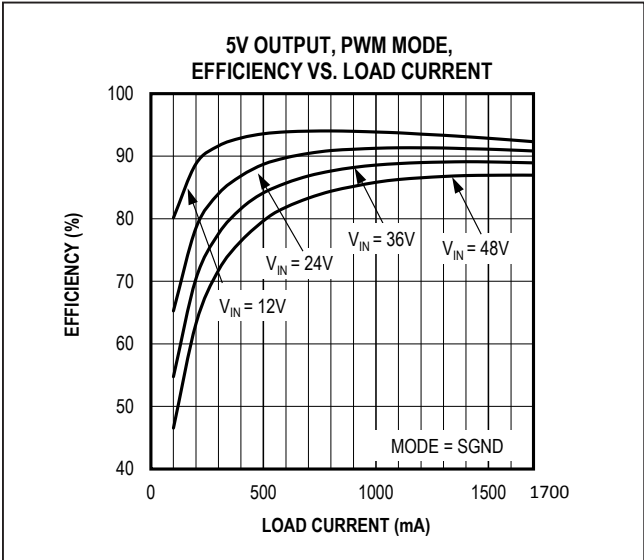
Figure 2. MAX17505 5V Output Efficiency (PWM Mode)
