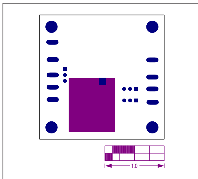
Figure 18. MAX17505 5V Output EV Kit Component Placement Guide—Bottom Solder Mask
