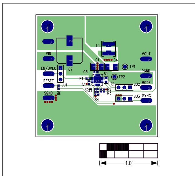
Figure 13. MAX17505 5V Output EV Kit Component Side PCB layout
