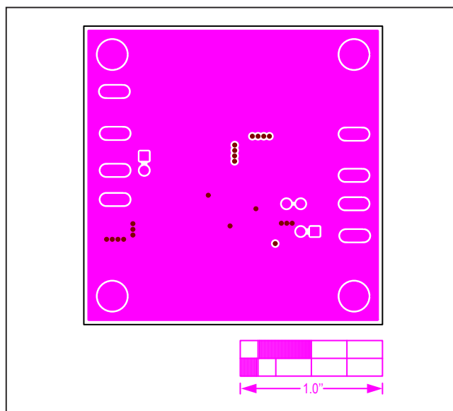
Figure 15. MAX17505 5V Output EV Kit PCB Layout—Inner Layer 2
