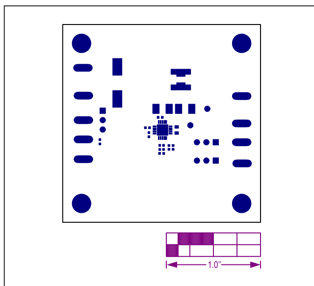
Figure 17. MAX17505 5V Output EV Kit Component Placement Guide—Top Solder Mask
