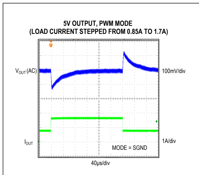
Figure 10. MAX17505 5V Output, 0.85A to 1.7A Load Transient
