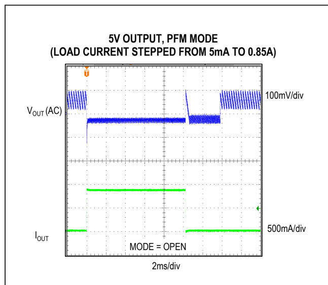
Figure 8. MAX17505 5V Output, 5mA to 0.85A Load Transient (PFM Mode)
