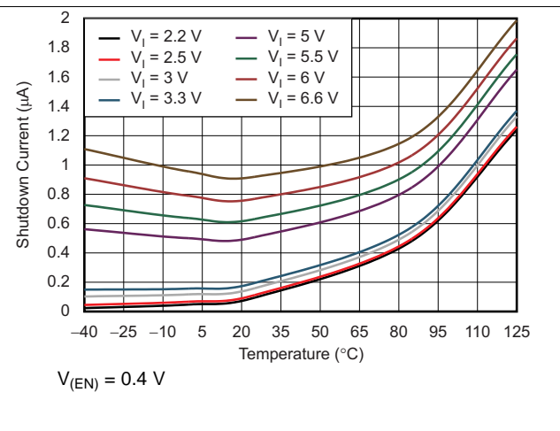
Figure 12. Shutdown Current vs Temperature
