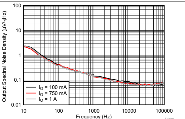
Figure 23. Output Spectral Noise Density vs Frequency (RMS noise (100 Hz to 100 kHz))
