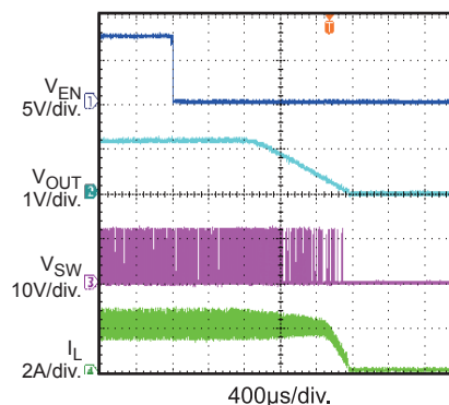
Shutdown through V_{EN} I_{OUT} = 2A
