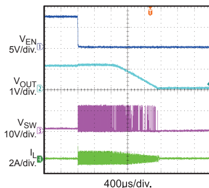
Shutdown through V_{EN} I_{OUT} = 0A
