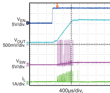
Start-up through V_{EN} I_{OUT} = 0A
