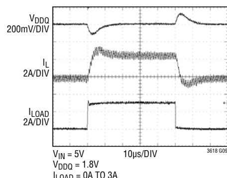
Load Step Transient with FCM Internal Compensation
