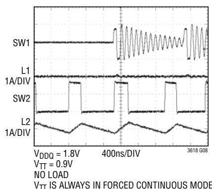
Pulse-Skipping Mode
