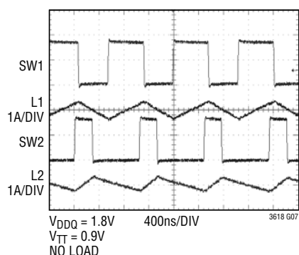
Forced Continuous Mode Operation (FCM)
