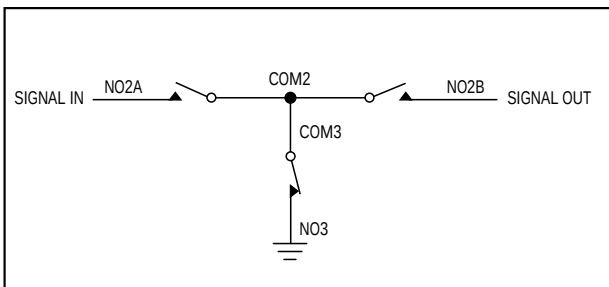
Figure 7. T-Switch Configuration
