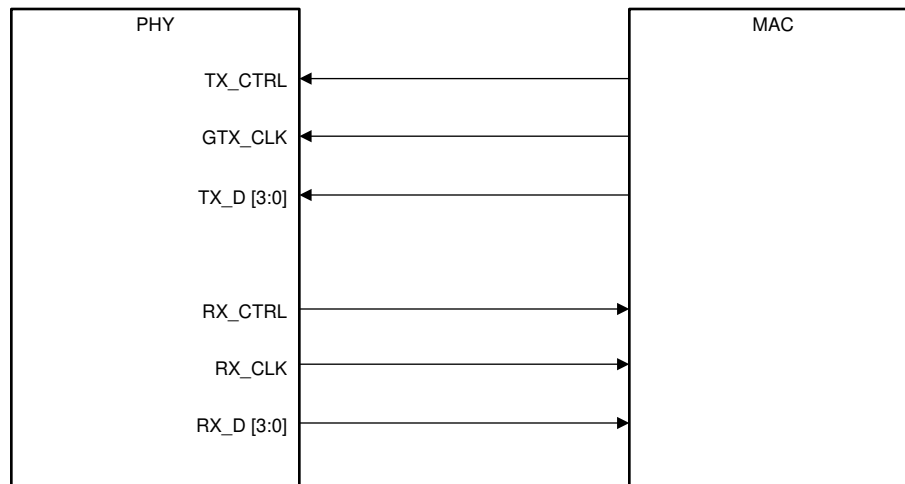
Figure 16. RGMII Connections
