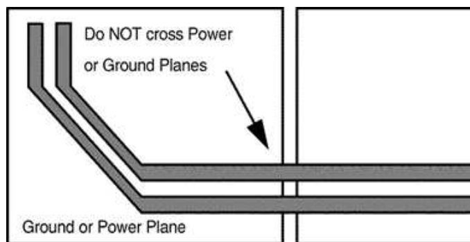
Figure 36. Differential Signal Pair-Plane Crossing
