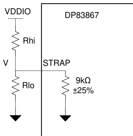
Figure 21. Strap Circuit
