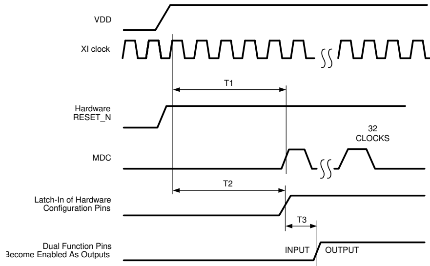
Figure 1. Power-Up Timing
