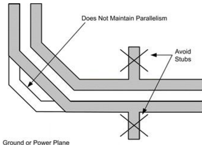
Figure 35. Avoiding Stubs in a Differential Signal Pair
