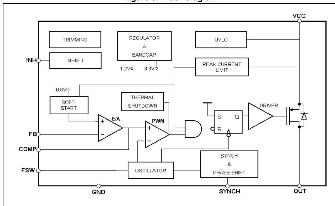
Figure 3. Block diagram
