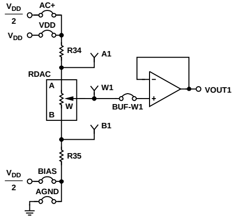
Figure 2. DAC
