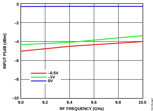
Figure 42. Input Power for 1 dB Compression (P1dB) vs. RF Frequency at Various Control Voltages
