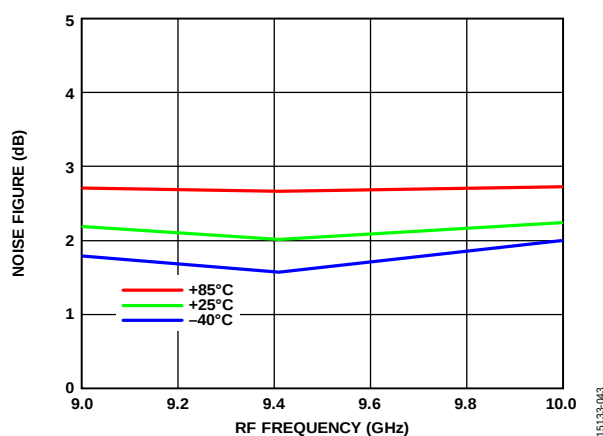
Figure 43. Noise Figure vs. RF Frequency over Temperature
