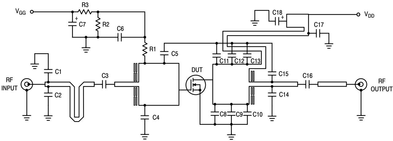
Figure 1. Broadband GSM 900 Test Circuit Schematic
