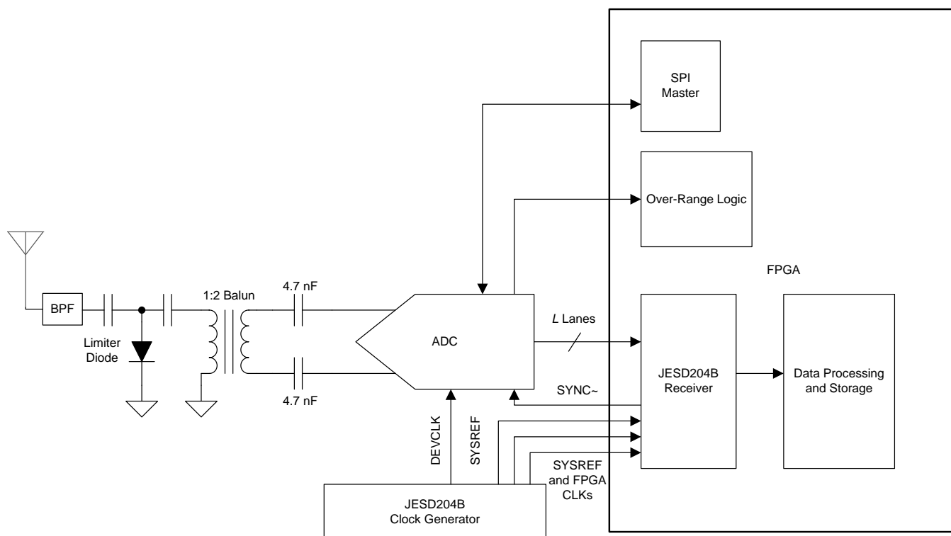
Figure 94. Simplified Schematic
