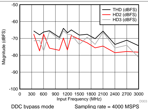
Figure 18. THD, HD2, HD3 vs Input Frequency
