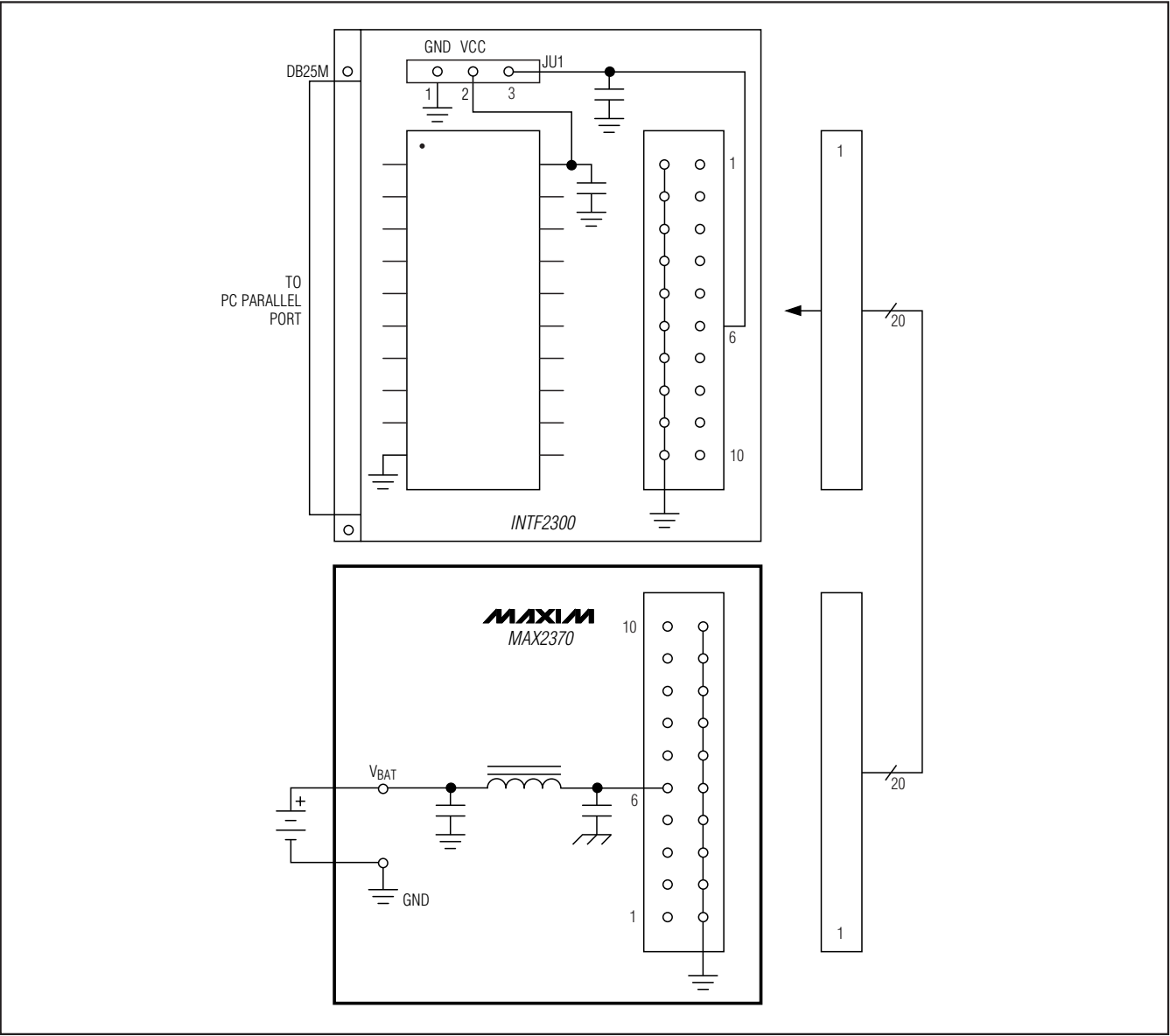
Figure 1. INTF2300 with MAX2370 EV Kit Providing Filtered Supply
