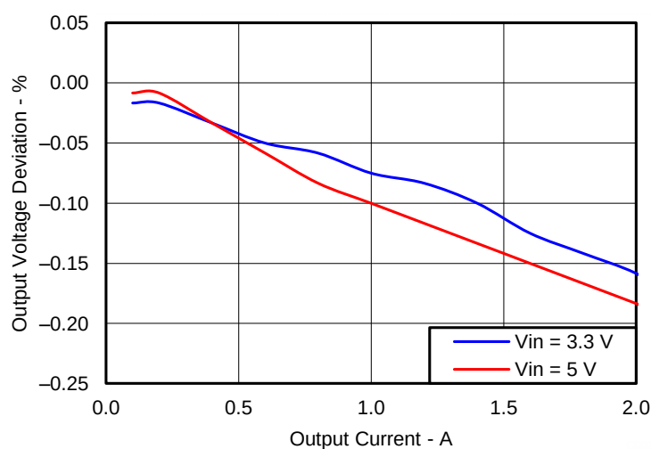
Figure 2. TPS57114EVM Load Regulation
