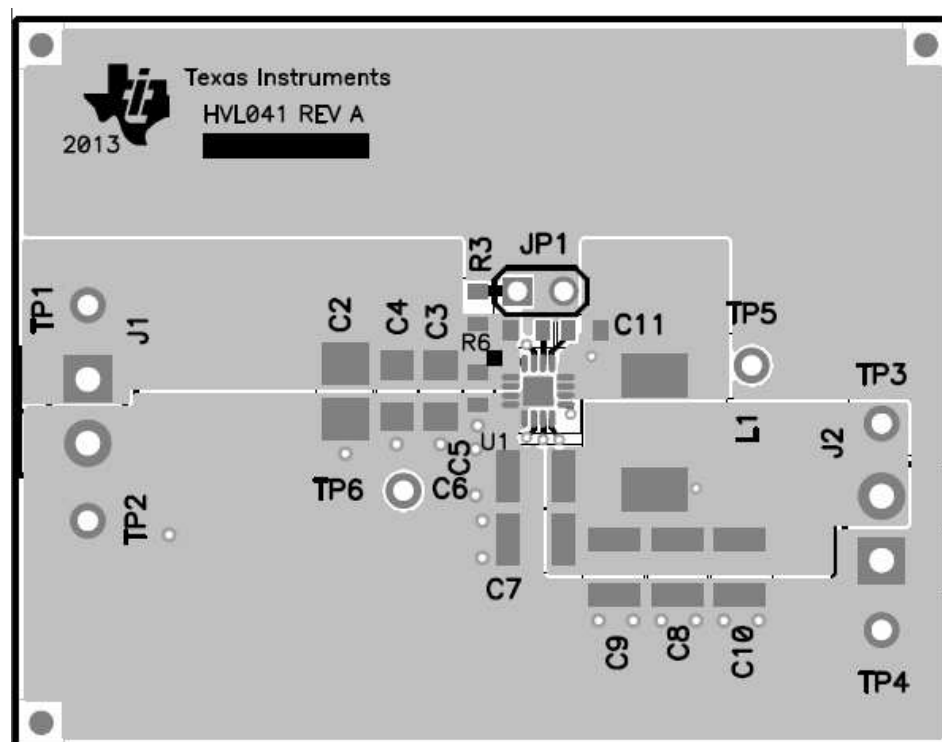
Figure 11. TPS57114EVM Top-Side Assembly
