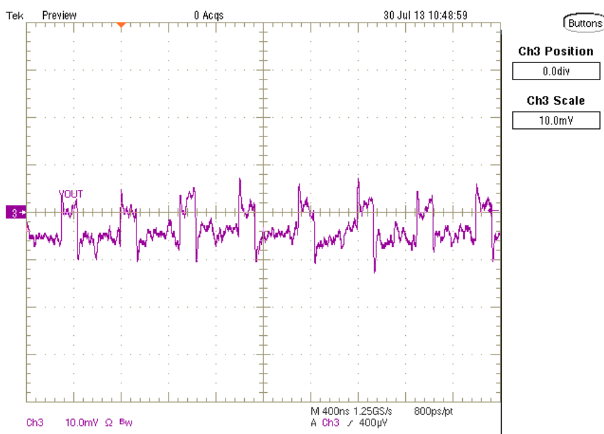
Figure 6. TPS57114EVM Output Ripple
