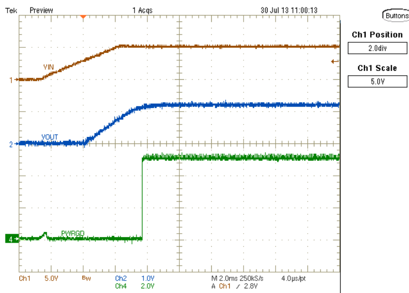
Figure 7. TPS57114EVM Startup Relative to V_{IN}
