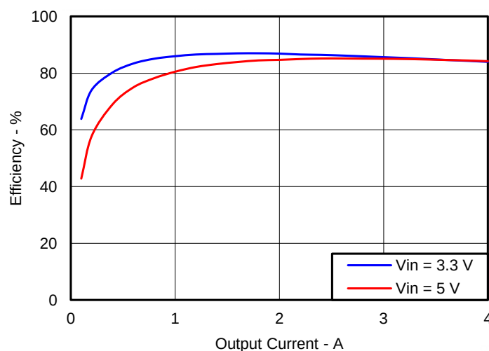
Figure 1. TPS57114EVM Efficiency
