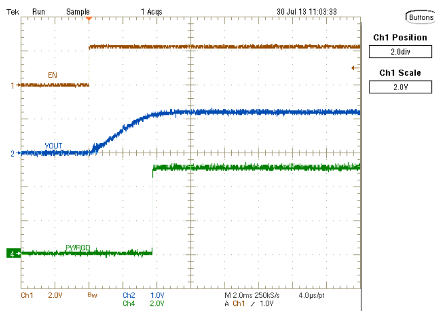
Figure 8. TPS57114EVM Startup Relative to Enable
