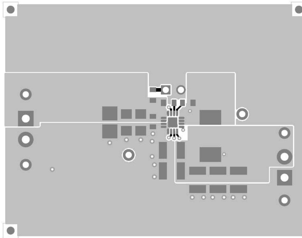
Figure 9. TPS57114EVM Top-Side Layout
