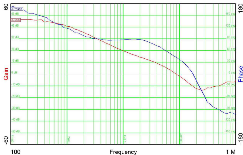
Figure 5. TPS57114EVM Loop-Response Measurement
