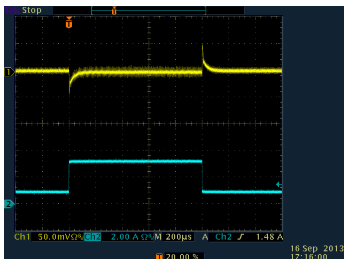
Figure 4. TPS57114EVM Load Transient
