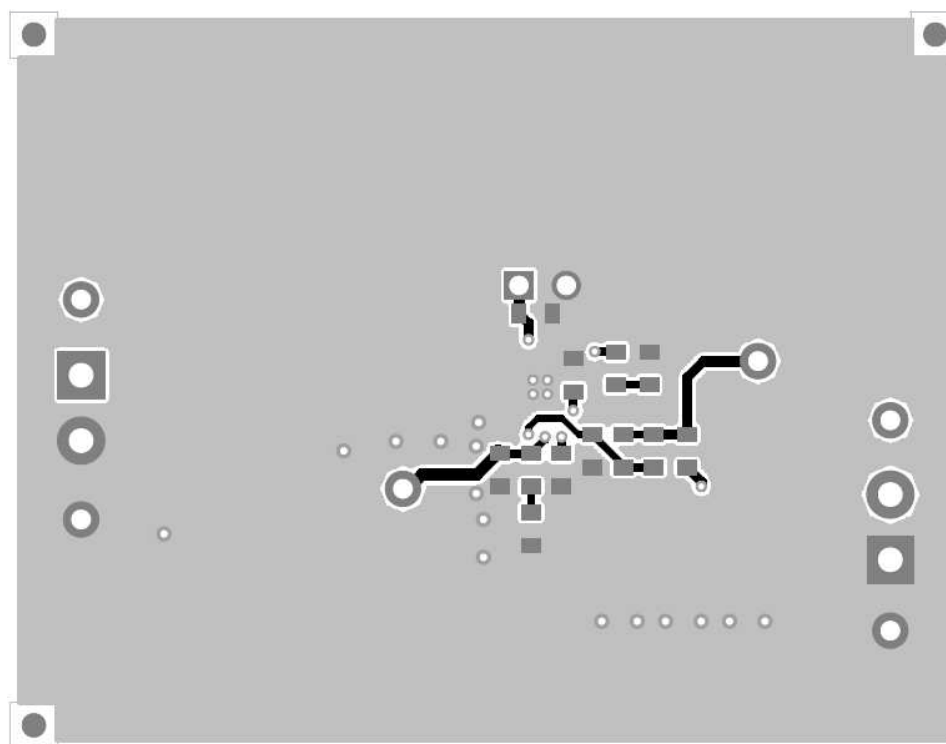
Figure 10. TPS57114EVM Bottom-Side Layout
