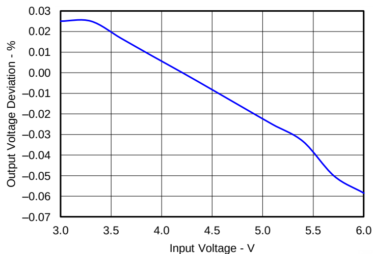
Figure 3. TPS57114EVM Line Regulation
