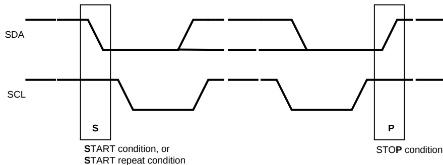
Figure 36. Start and Stop Conditions
