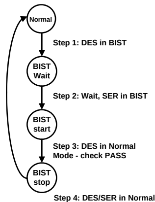
Figure 16. BIST Mode Flow Diagram
