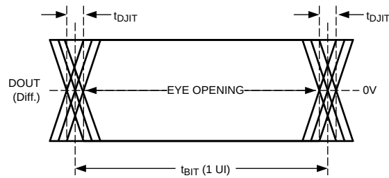
Figure 4. Serializer Output Jitter
