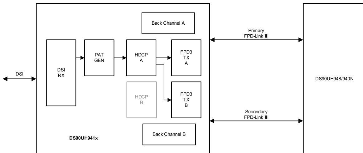
Figure 26. Dual-Link, 1:2 Mode
