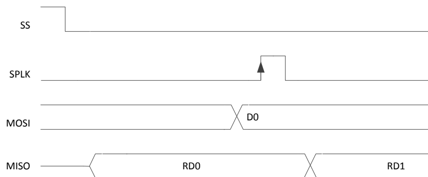
Figure 12. Reverse Channel SPI Read
