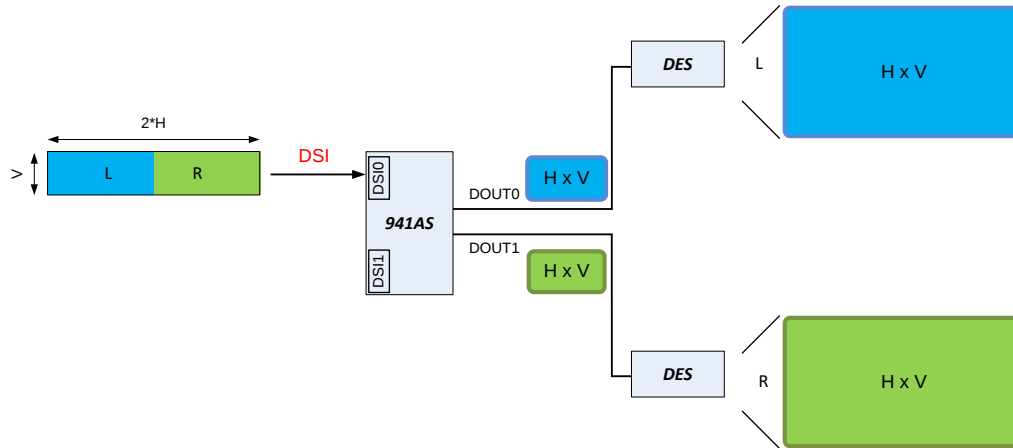
Figure 21. Splitting at Serializer Option
