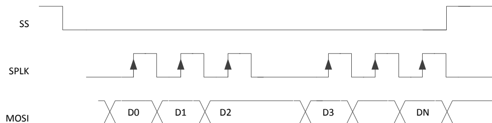
Figure 11. Reverse Channel SPI Write
