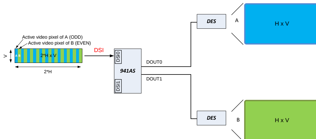
Figure 30. Alternate Pixel Splitting
