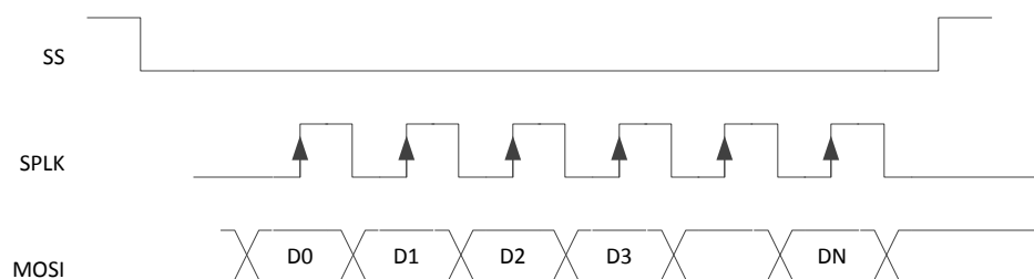
Figure 9. Forward Channel SPI Write
