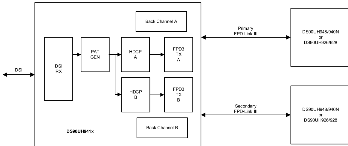
Figure 27. Replicate Mode
