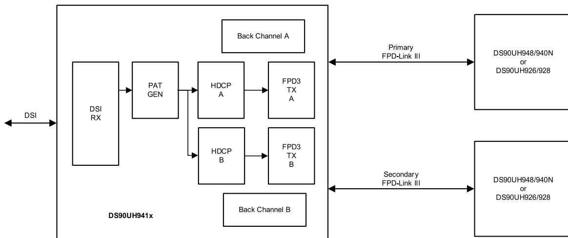
Figure 28. Splitter Mode
