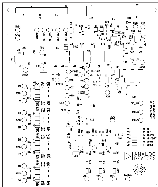
Figure 36. Evaluation Board Silkscreen
