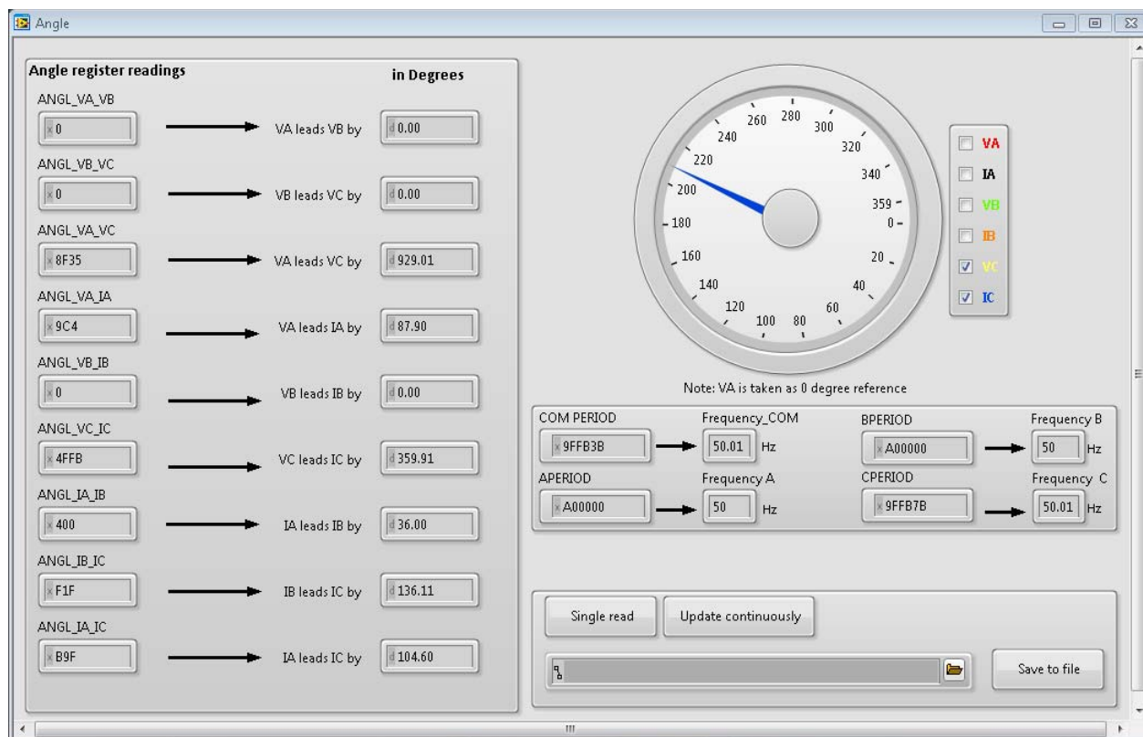
Figure 23. Angle Window
