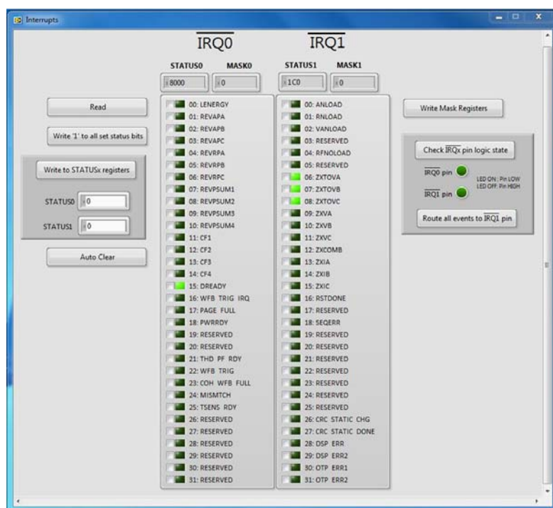
Figure 27. Interrupts Window
