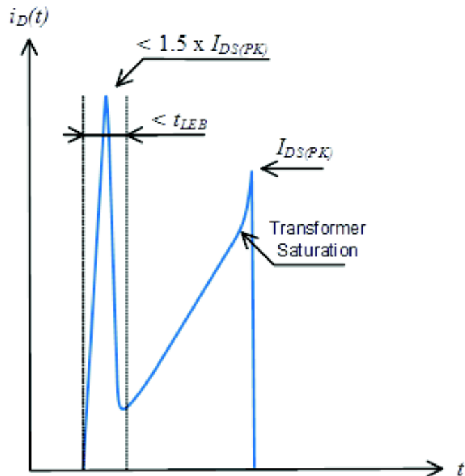
Figure 4. Spike Limits
