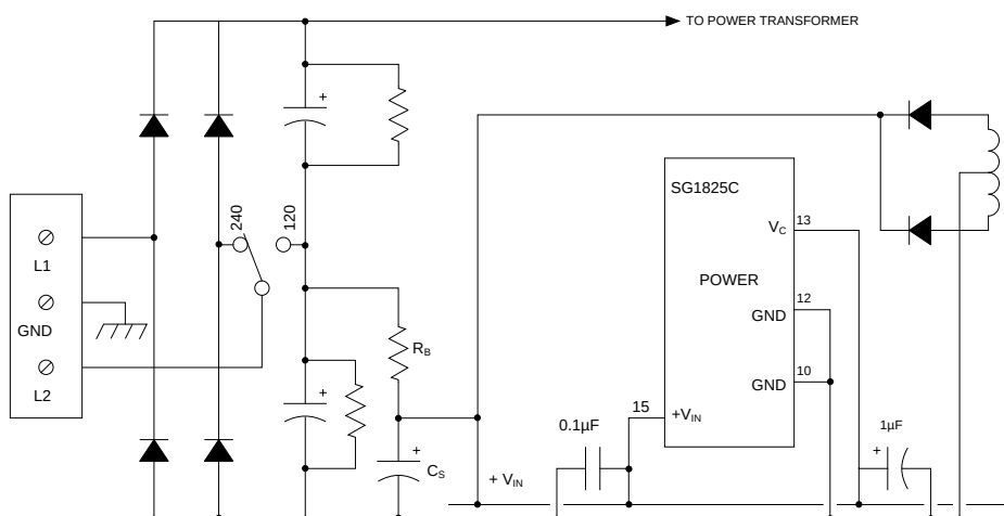
Figure 5 • Micropower Startup
