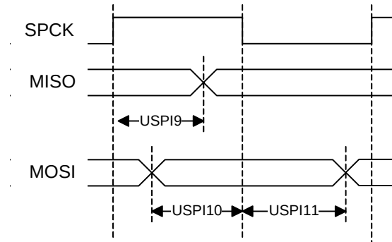
Figure 35-12. USART in SPI Slave Mode with (CPOL= CPHA= 0) or (CPOL= CPHA= 1)
