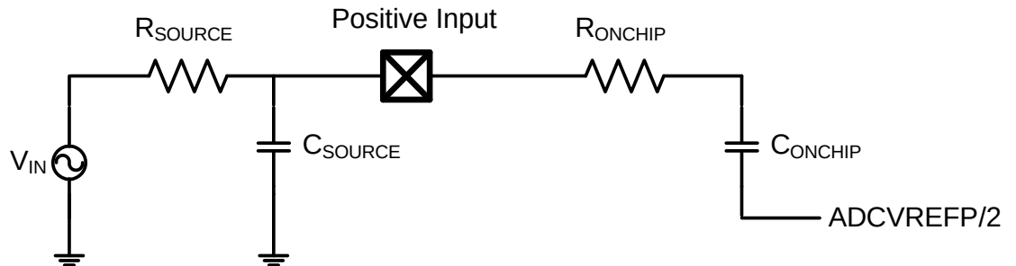
Figure 35-8. ADC Input
