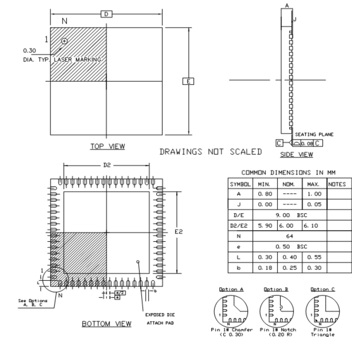
Figure 36-5. QFN-64 Package Drawing
