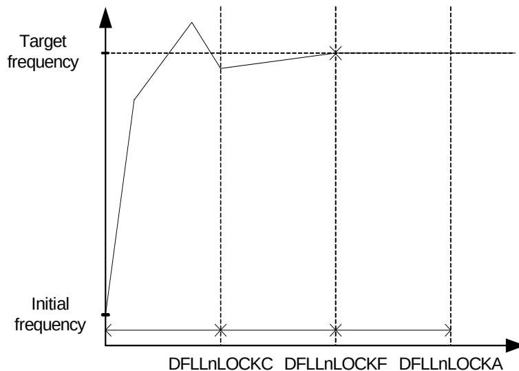
Figure 14-4. DFLL Locking in Closed loop
