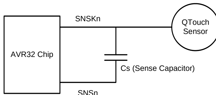
Figure 31-2. CAT Touch Connections
