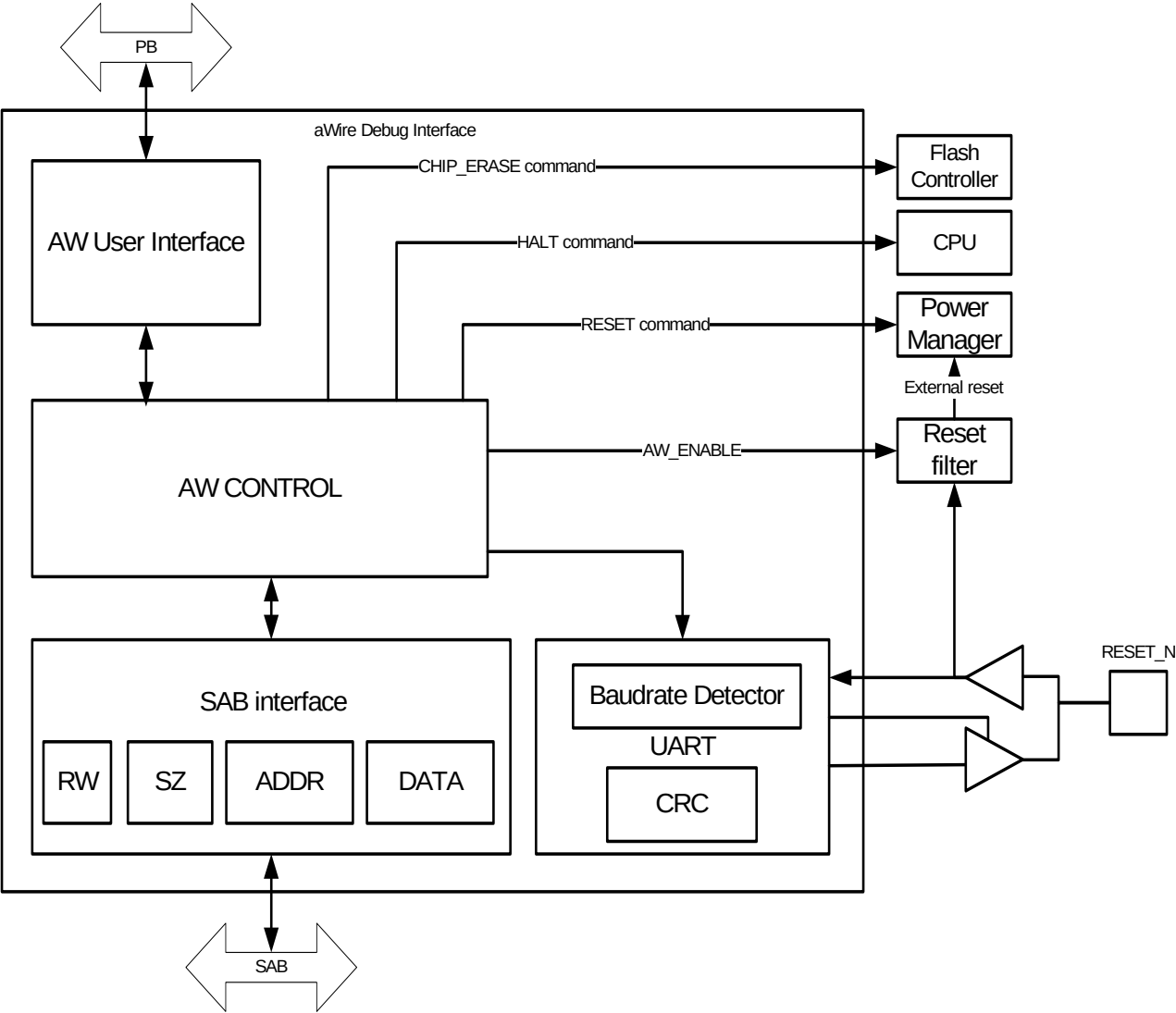
Figure 34-8. aWire Debug Interface Block Diagram
