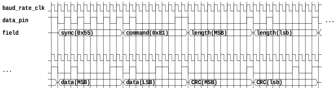
Figure 34-9. Example Command
