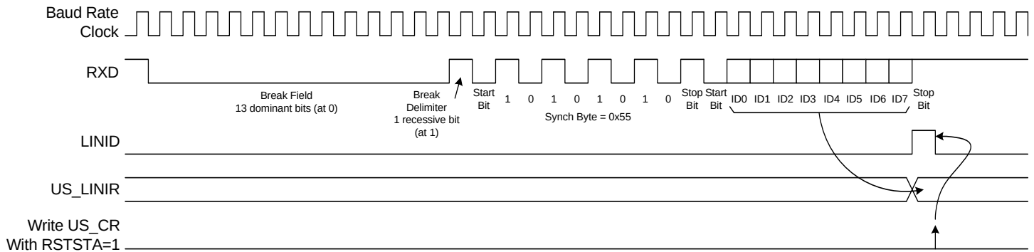
Figure 20-22. Header Reception
