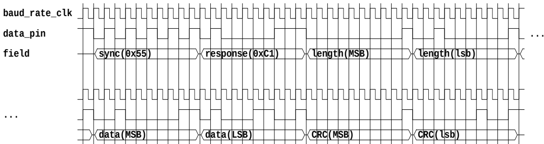
Figure 34-10. Example Response
