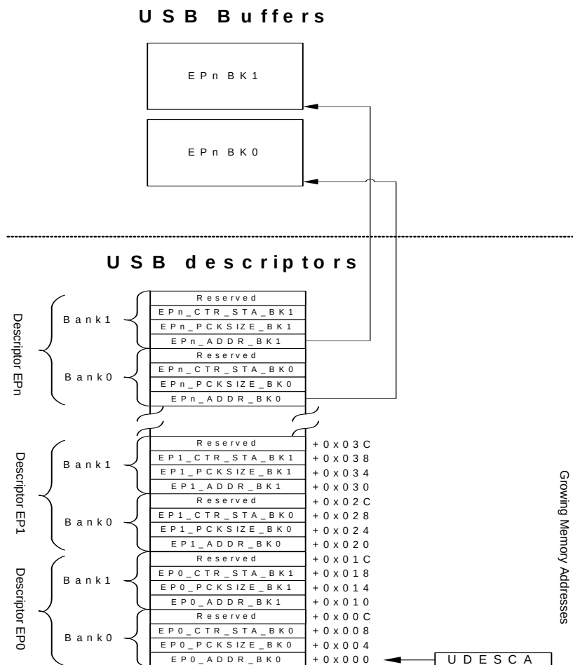
Figure 8-5. Memory organization
