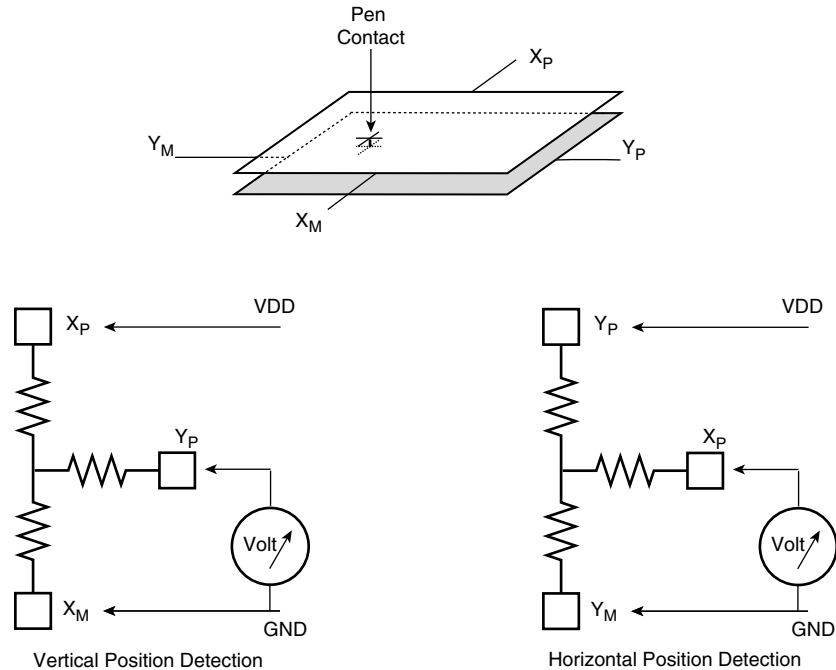
Figure 29-2. Resistive Touch Screen Position Measurement
