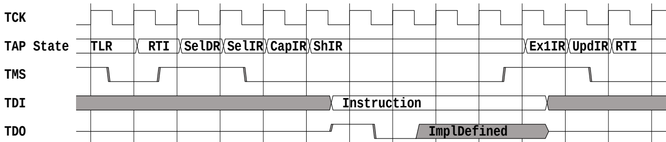
Figure 34-7. Scanning in JTAG Instruction
