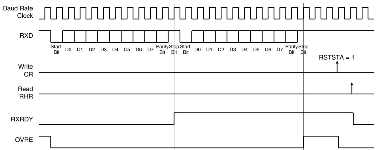
Figure 20-9. Receiver Status
