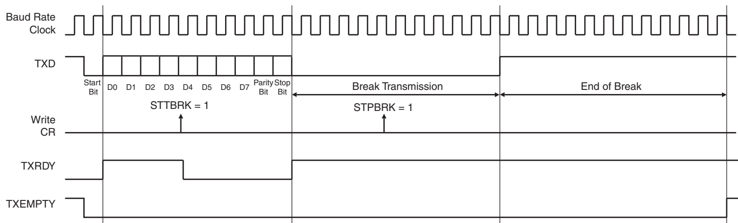
Figure 20-14. Break Transmission
