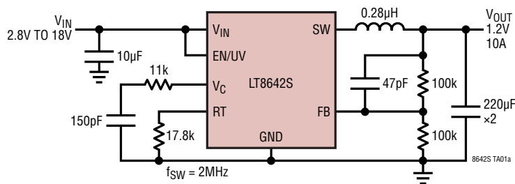
1.2V 10A Step-Down Converter
