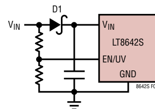
Figure 7. Reverse V_{IN} Protection
