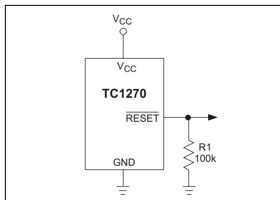
FIGURE 4-2: Ensuring \overline{\text{RESET}} Valid to V_{CC} = 0\text{V} .
